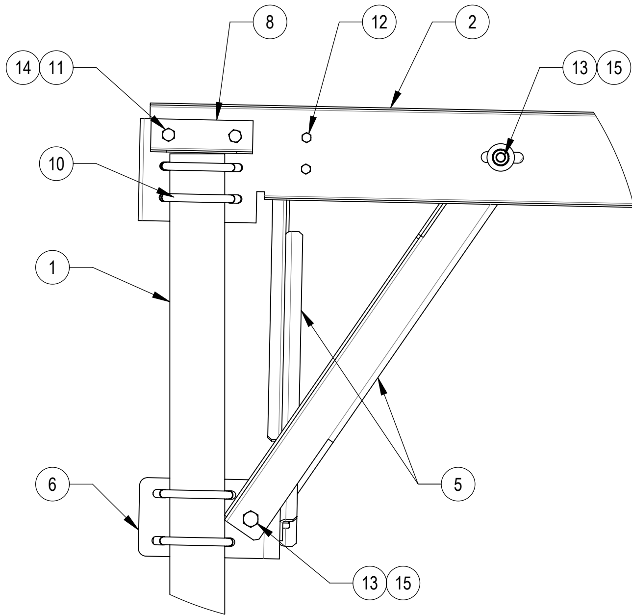
DETAIL A SCALE 1 : 6
