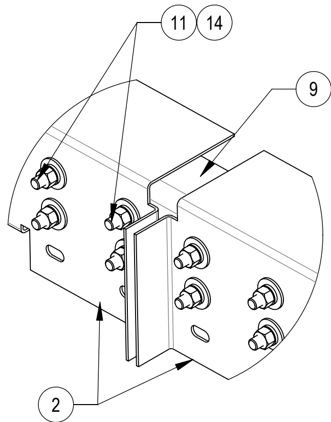
DETAIL C SCALE 1 : 4
