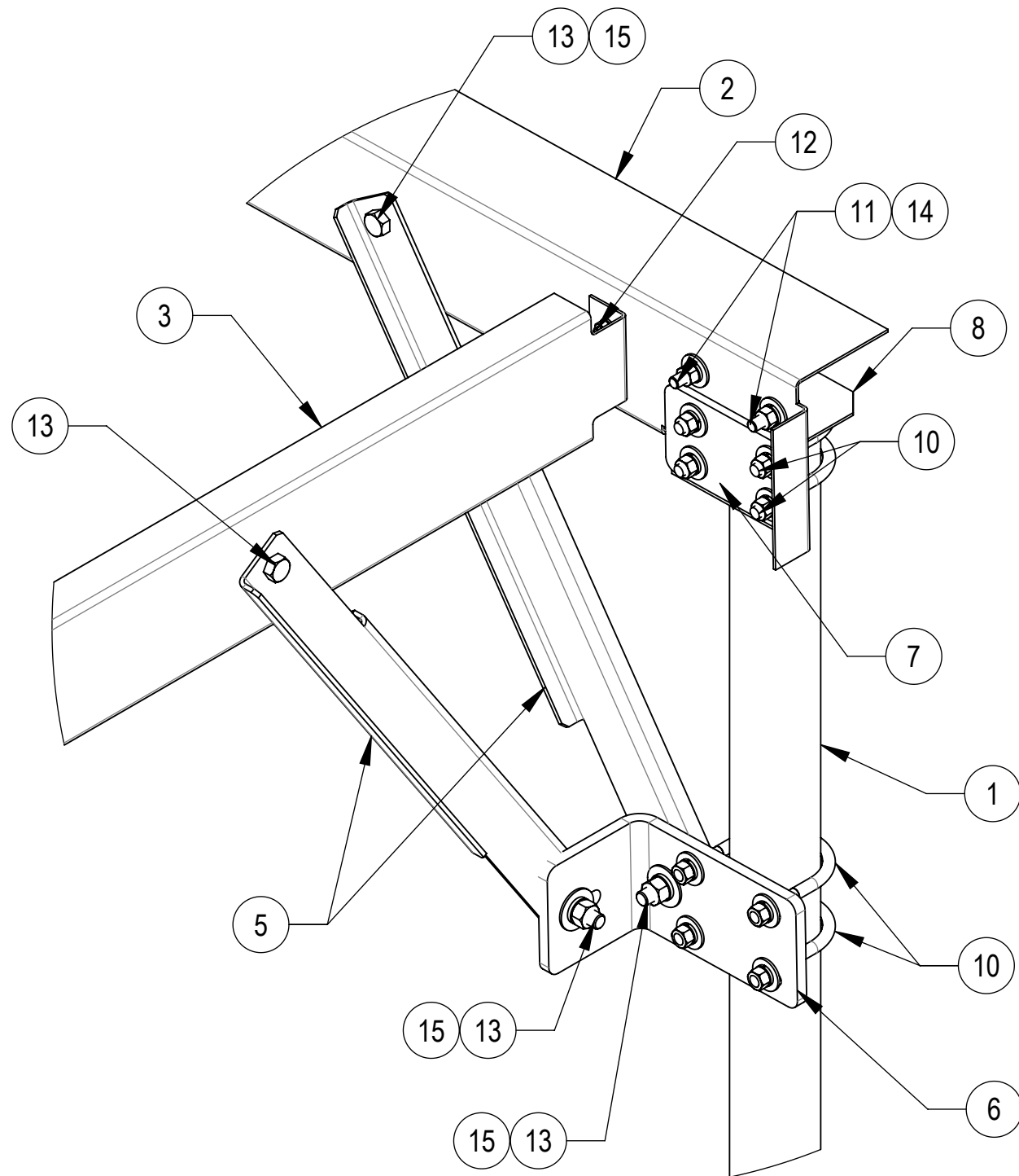
DETAIL B SCALE 1 : 6
