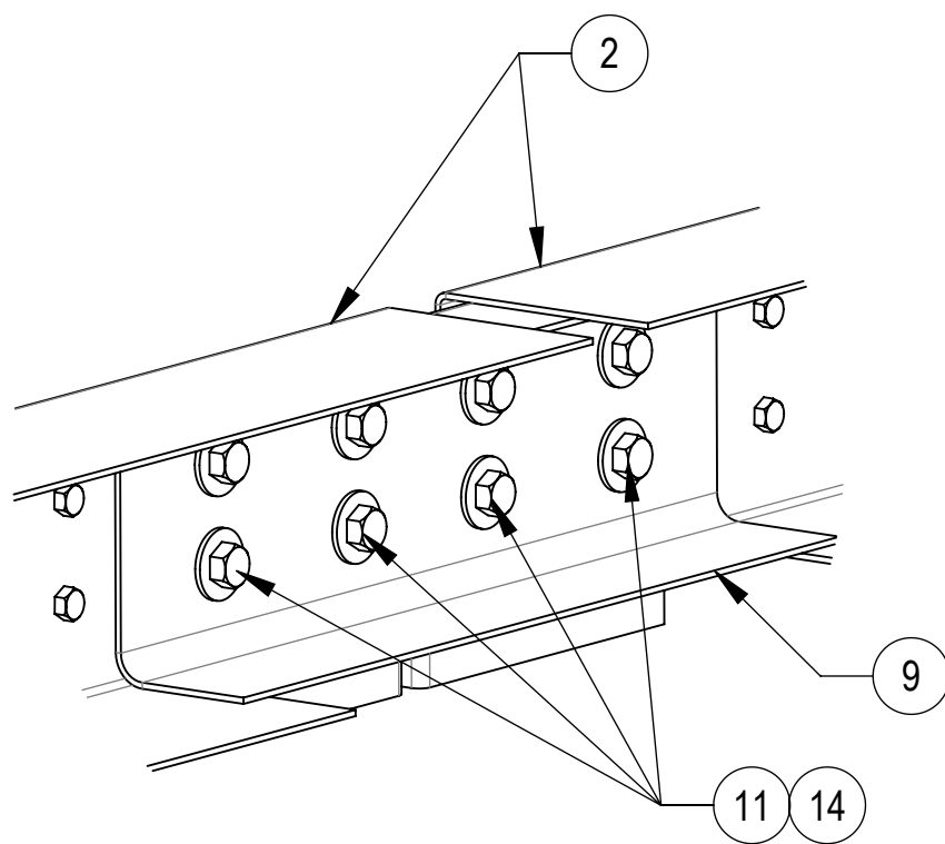
DETAIL C BACK VIEW SCALE 1 : 4
