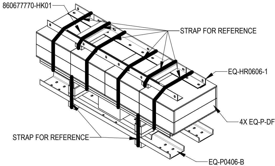
PACKING VIEW
