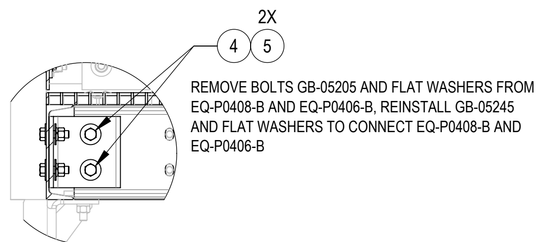
DETAIL B SCALE 1 : 8 (2 PLACES)
