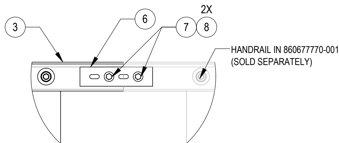
DETAIL C SCALE 1 : 6 (3 PLACES) (HIDE ICE CANOPY FOR CLARITY)
