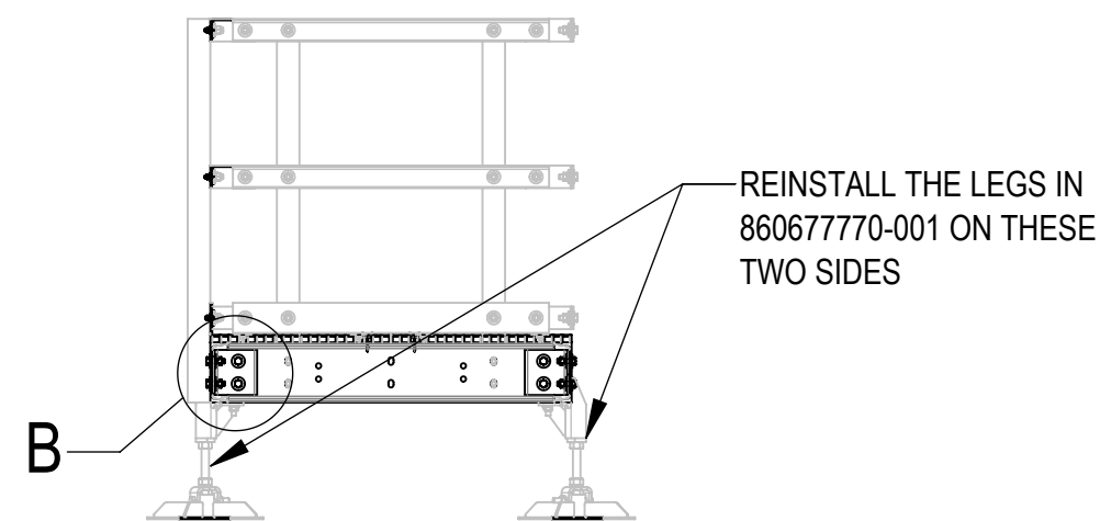
SECTION A-A (HIDE ICE CANOPY FOR CLARITY)
