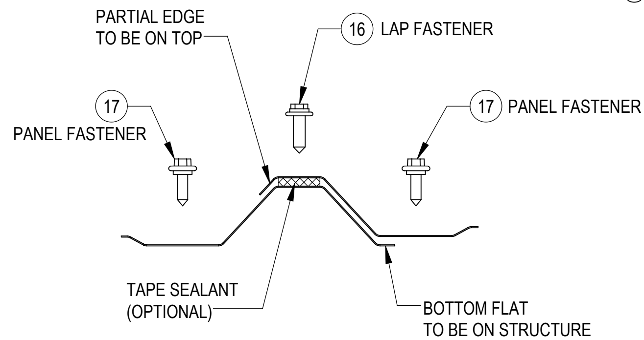
TYPICAL PANEL JOINT DETAIL
