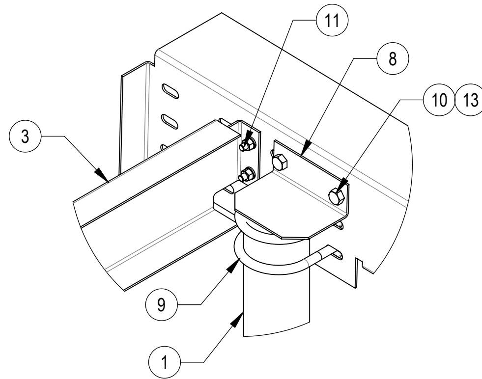
DETAIL E SCALE 1 : 5
