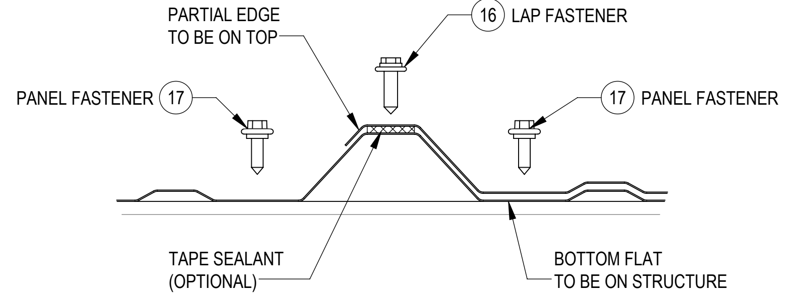
TYPICAL PANEL JOINT DETAIL
