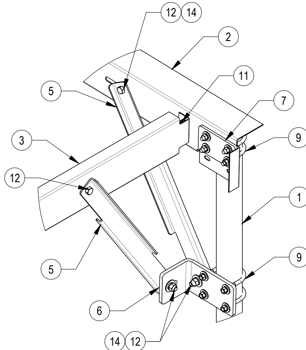
DETAIL B SCALE 1 : 8
