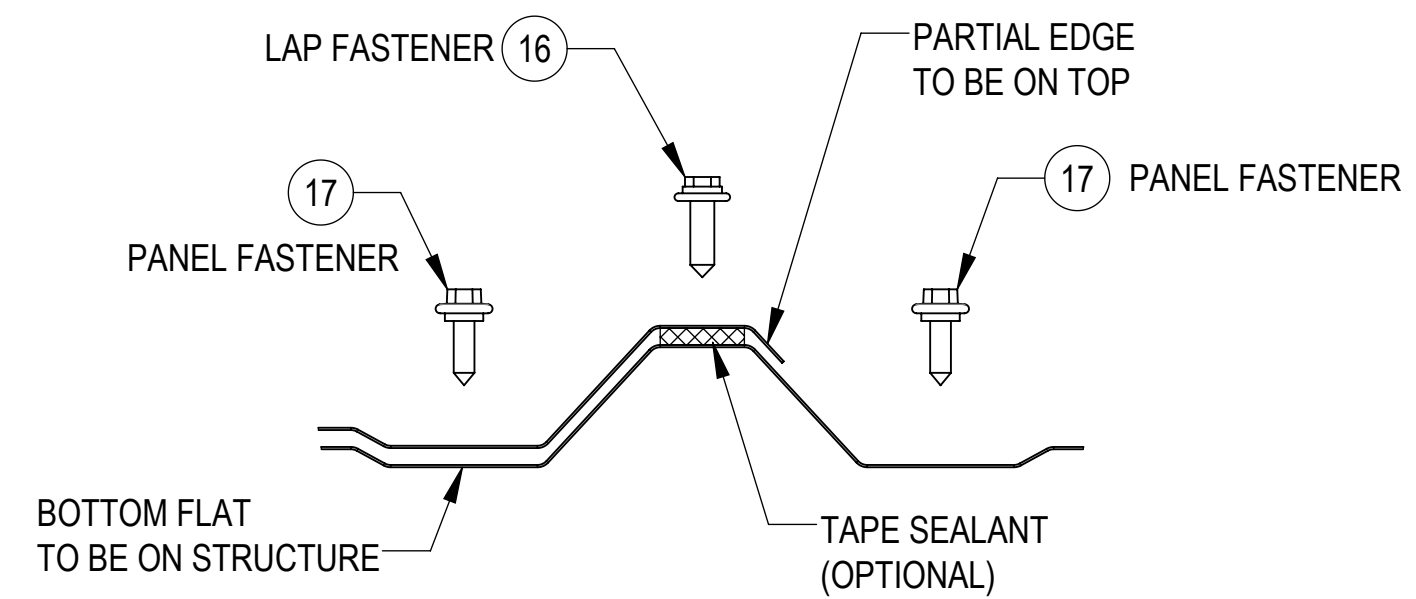
TYPICAL PANEL JOINT DETAIL
