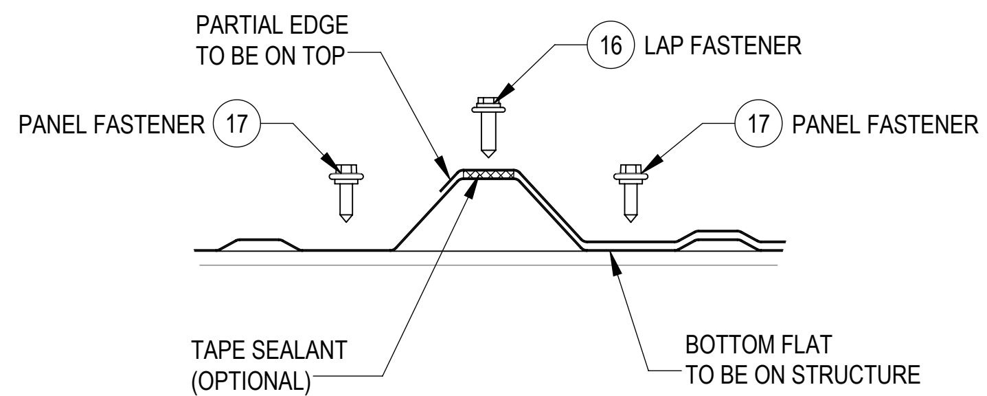
TYPICAL PANEL JOINT DETAIL
