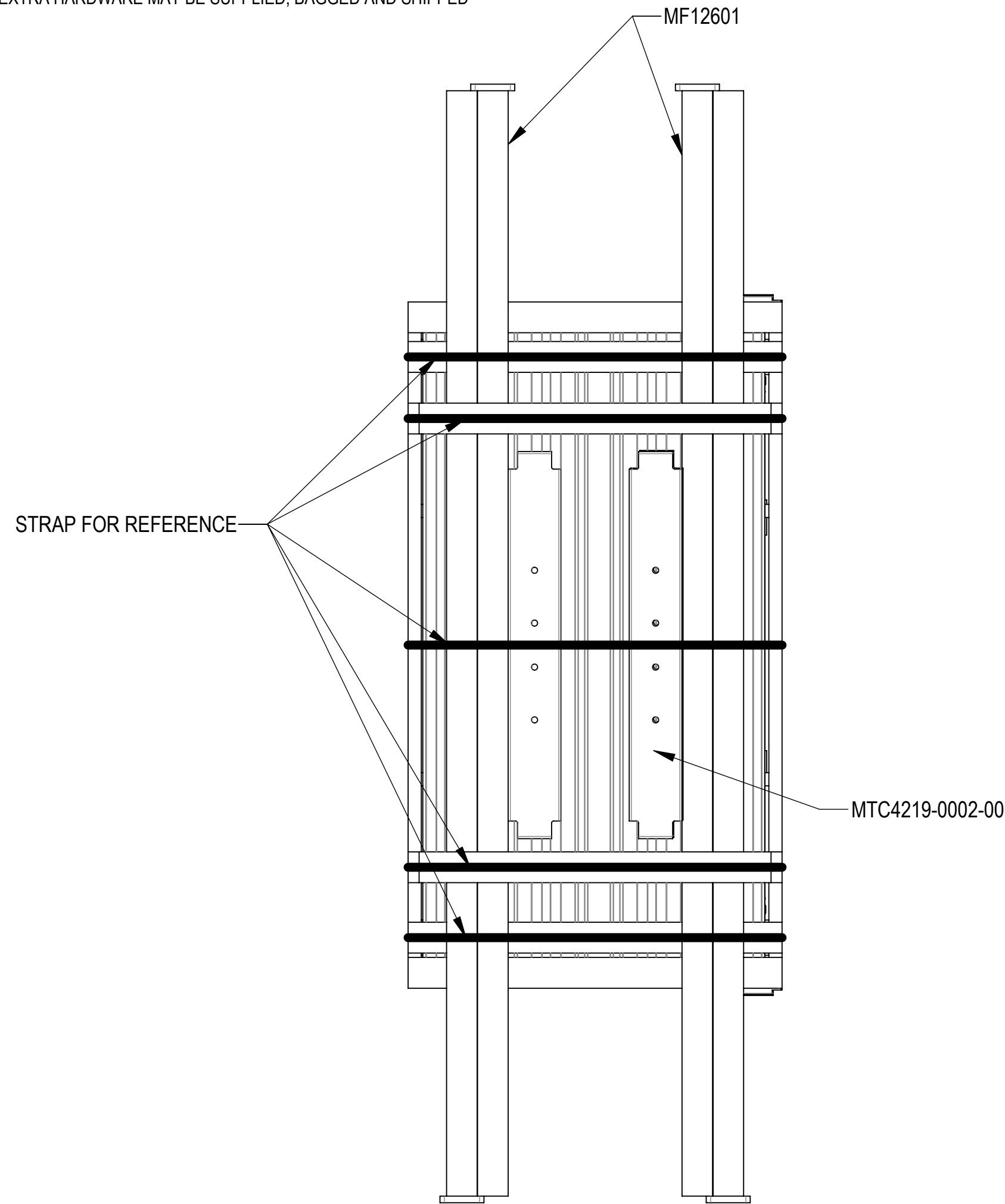
BOTTOM VIEW
