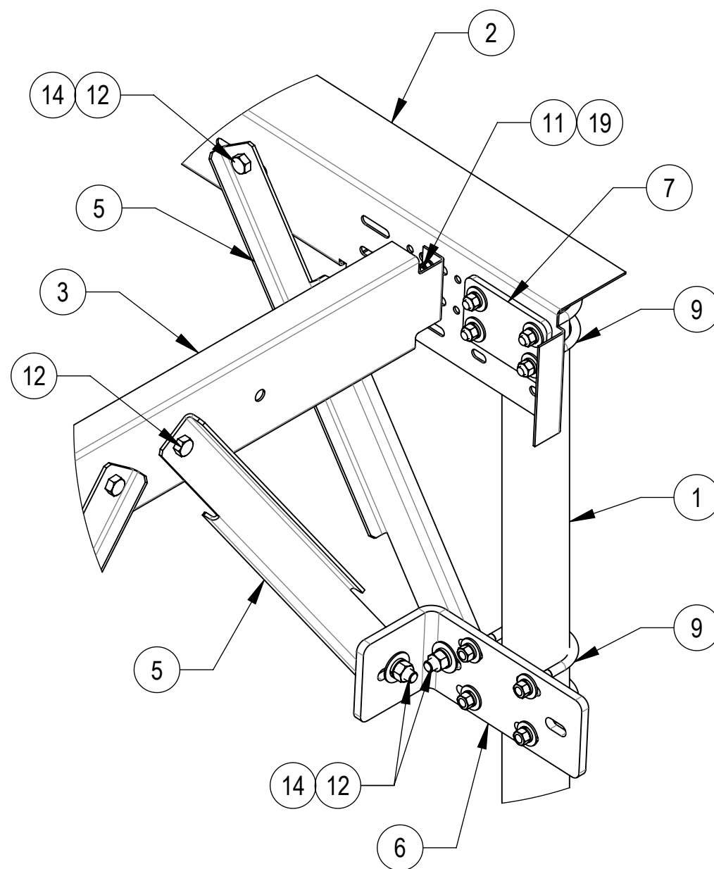
DETAIL B SCALE 1 : 7
