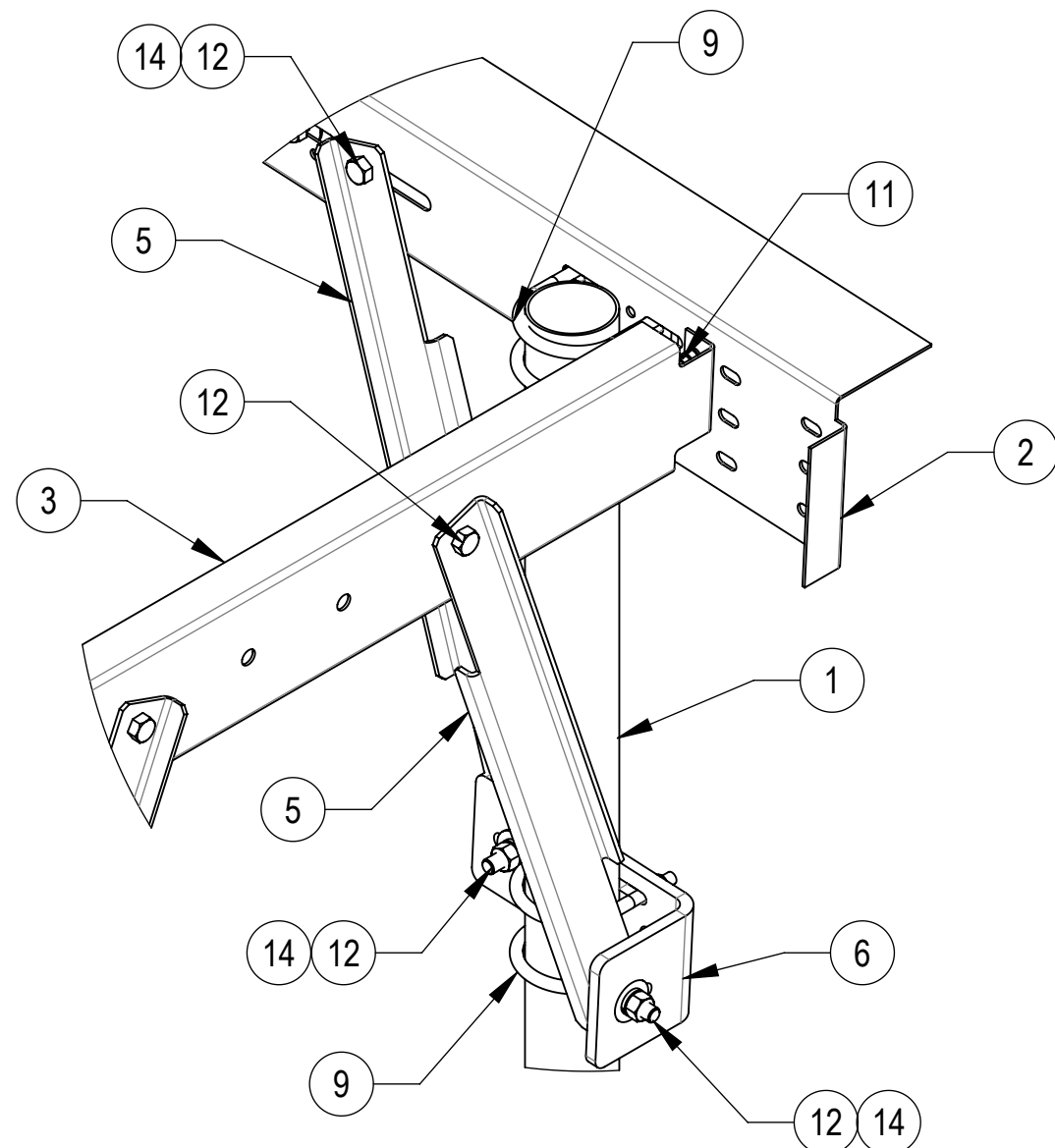
DETAIL D SCALE 1 : 7
