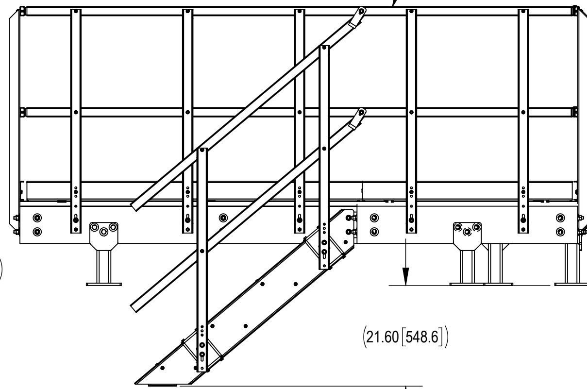
STAIR WITH EQP0404L-DSH & EQP0404LHR-DSH PLATFORM (SOME PARTS OF PLATFORM ARE HIDDEN FOR CLARITY)
