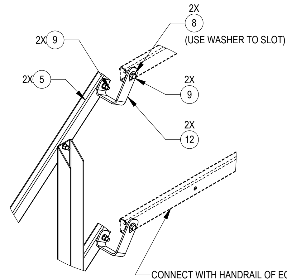
DETAIL XB SCALE 1:7
