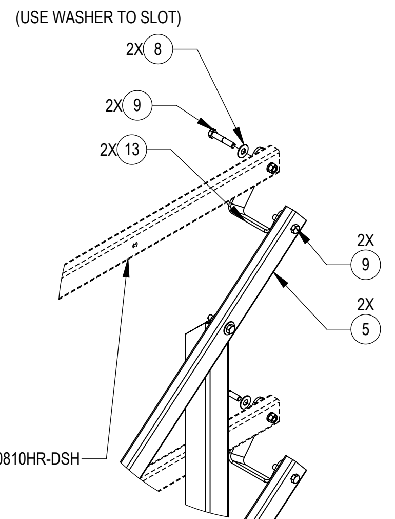
DETAIL XC SCALE 1:7
