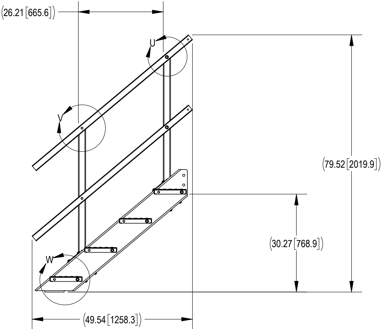
SECTION X-X SCALE 1 : 18
