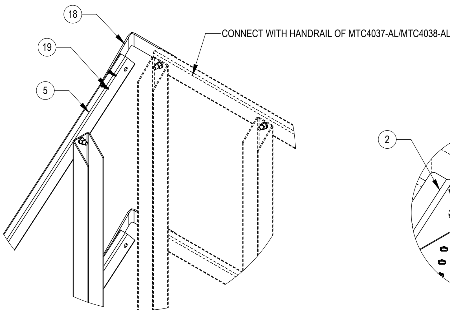
DETAIL F SCALE 1 : 6
