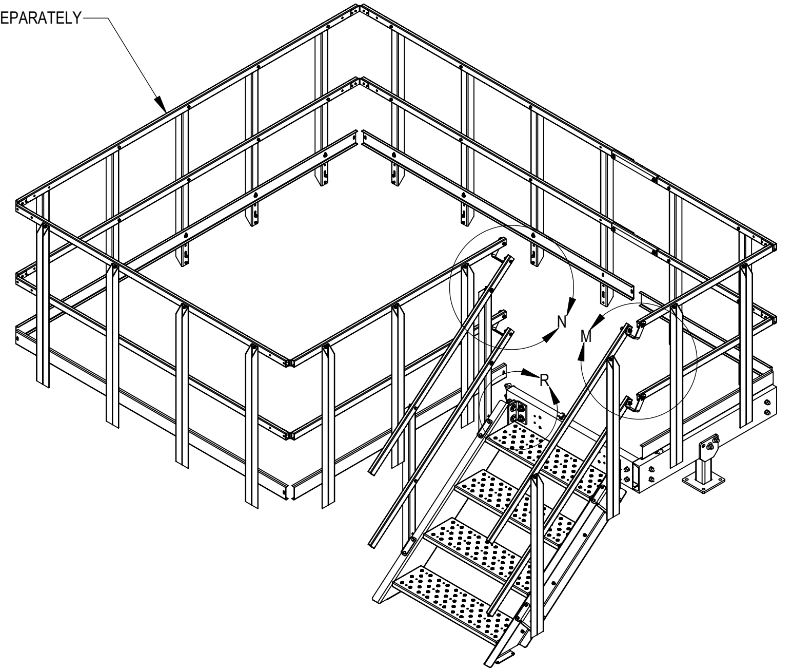
STAIR WITH EQP0404L-DSH & EQP0404LHR-DSH PLATFORM (SOME PARTS OF PLATFORM ARE HIDDEN FOR CLARITY)
