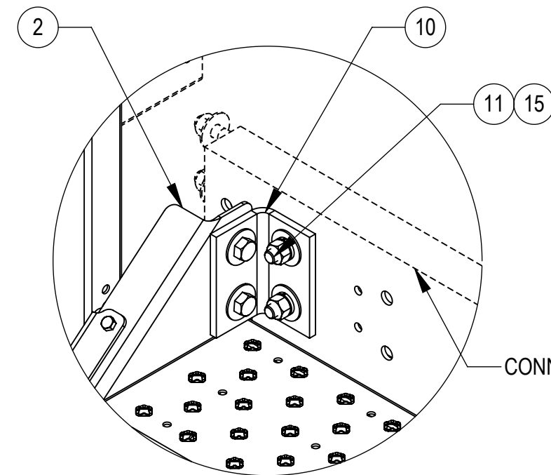
DETAIL R SCALE 1 : 6
