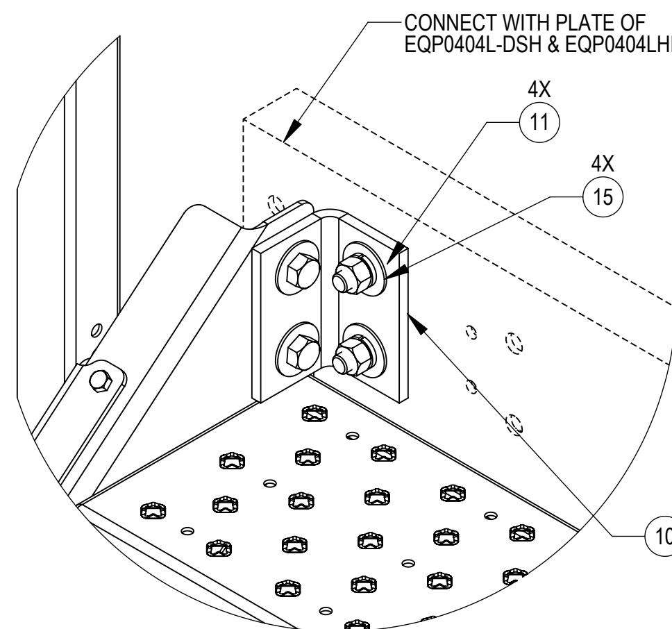
DETAIL XA SCALE 1:4
