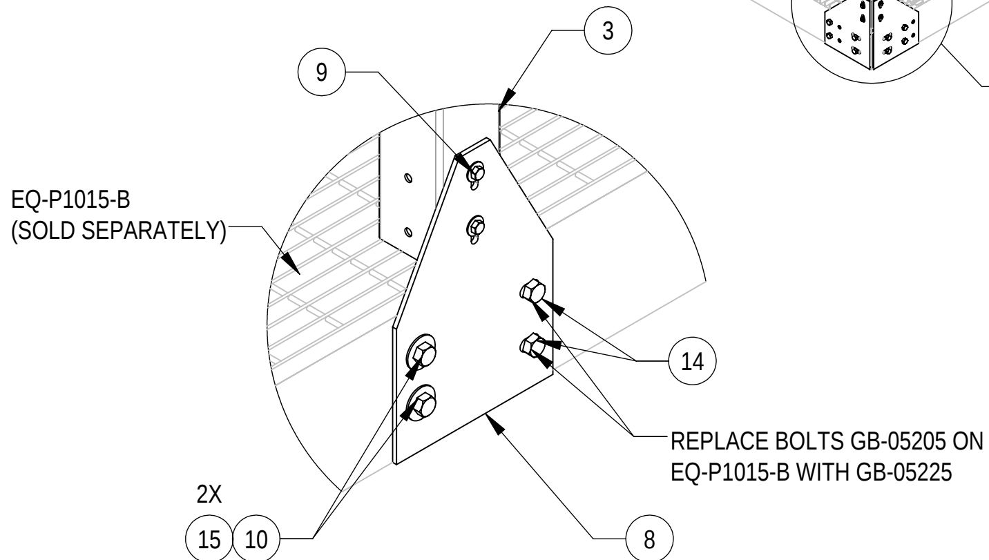
DETAIL D SCALE 1 : 6 (2 PLACES)
