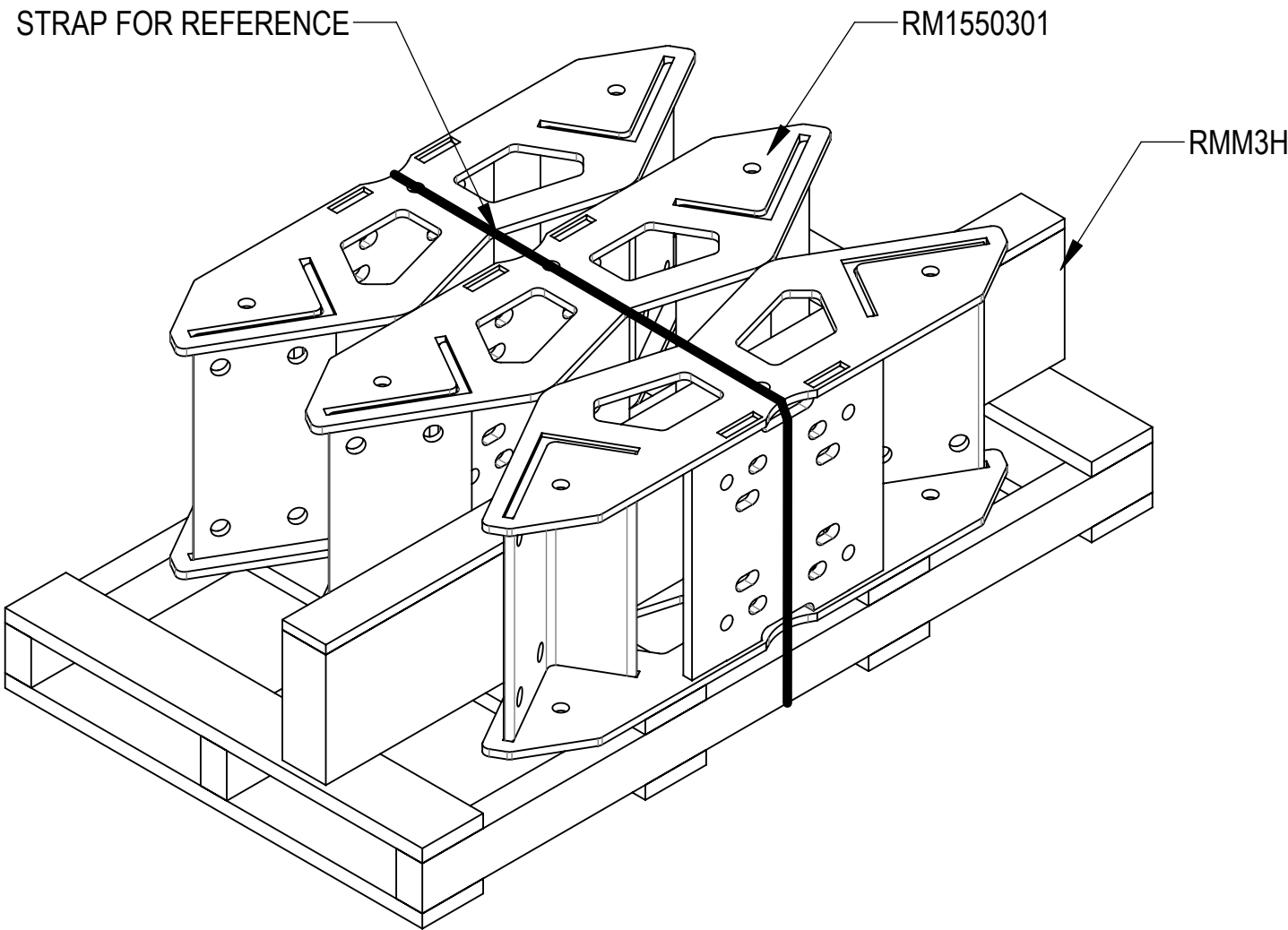
PACKAGING VIEW
