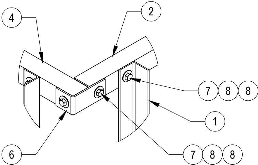
DETAIL A SCALE 1 : 8
