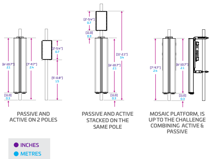
Figure 2—All FDD/TDD as well as 5G NR TDD bands can be deployed on a single pole
