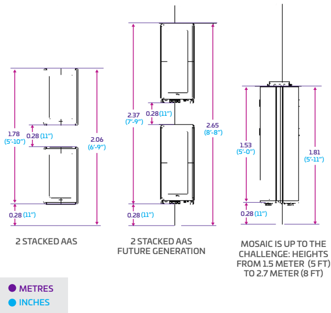
Figure 2—All FDD/TDD as well as 5G NR TDD bands can be deployed on a single pole
